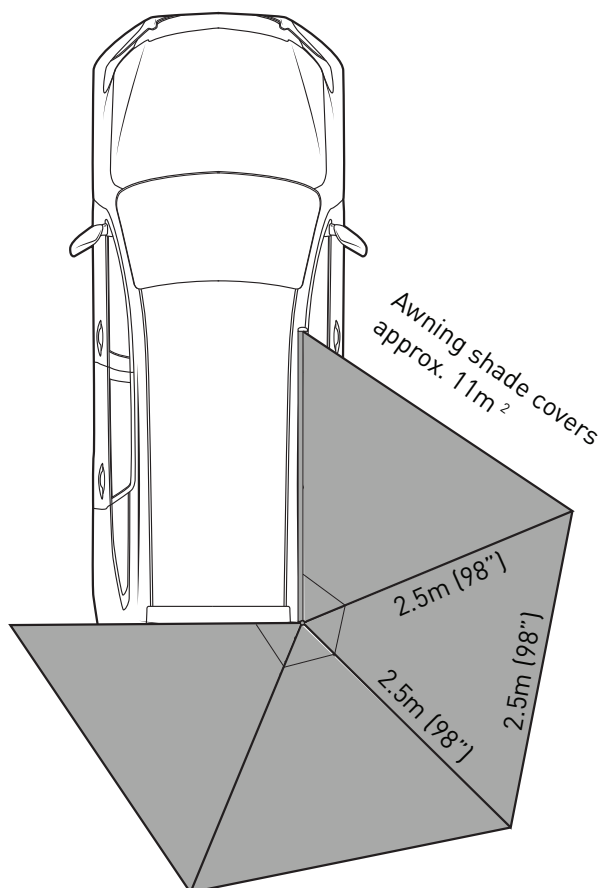
Overall Dimensions
